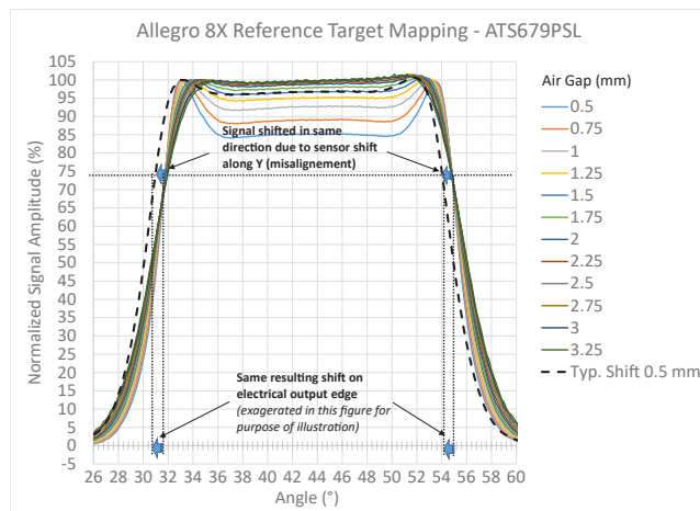
Figure 3: Signal shift due to sensor misplacement along Y axis – Full signal tooth is shifted.
