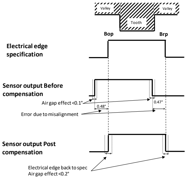
Figure 12: Benefits of threshold compensation method on sensor electrical output.
