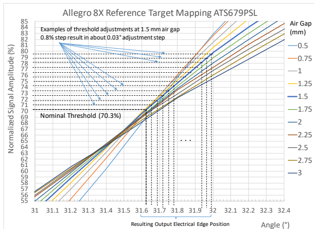
Figure 7: B_{OP} adjustment steps of ATS679PSL on Allegro 8X target ( B_{OP} is magnetic rising slope).
