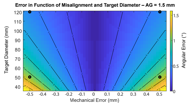
Figure 5: Electrical signal error (°) in function of mechanical misalignment along Y axis and target diameter. The small black circles correspond to the points marked in Figure 4.
