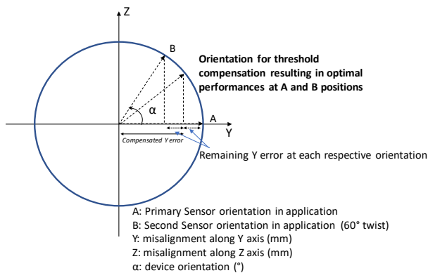
Figure 11: Effect of ATS679PSL orientation on Y axis misalignment.
