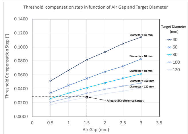
Figure 9: Effect of Air Gap and Target Diameter on ATS679PSL threshold compensation step.
