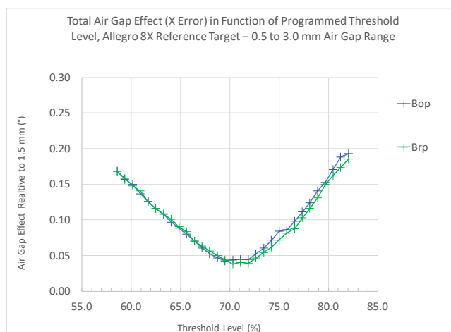
Figure 10: Effect of ATS679PSL threshold change on air gap effect (X error) with Allegro 8X target.
