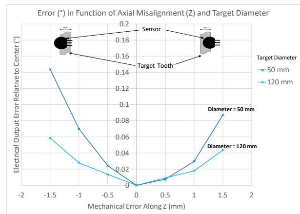
Figure 6: Electrical signal error (°) in function of mechanical misalignment along Z axis and target diameter. Non-symmetry is explained by the SL magnet non-symmetrical shape.
