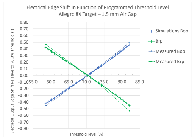
Figure 8: Effect of ATS679PSL threshold adjustment on relative electrical edge position with Allegro 8X target.
