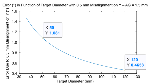
Figure 4: Electrical signal error in function of target diameter, at 0.5 mm of misplacement along Y axis.
