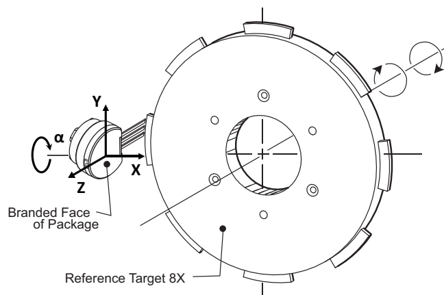
Figure 1: Axes definition for mechanical misalignments on Allegro's ATS679PSL in front of gear tooth target
