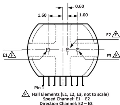
Figure 3: Hall element locations in SG package diagram.
