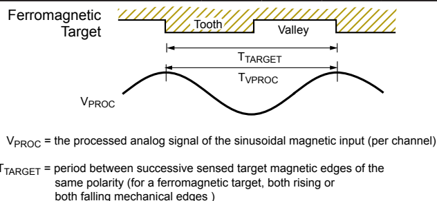
Figure 2: Definition of T_{TARGET} .
