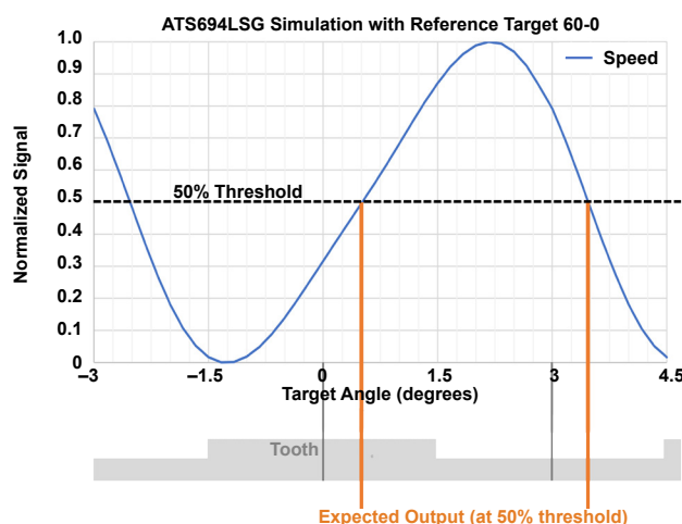
Figure 8: Predicted edge locations from simulation results.
