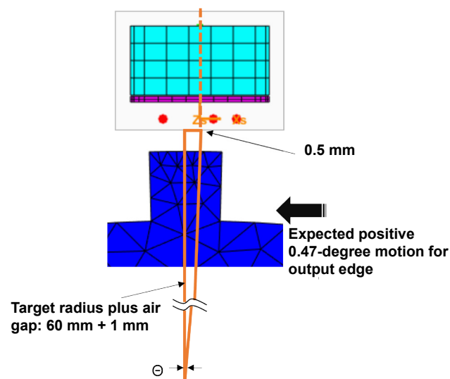
Figure 6: Computations of angular shift.
