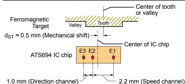
Figure 1: Definition of mechanical shift of switch point.
