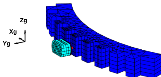
Figure 4: Isometric view.
