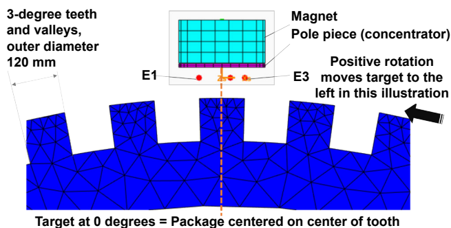
Figure 5: Simulation elements — Zero degrees is established with the SG package centered on the tooth. Positive rotation is defined as the target passing from E3 to E1 (Pin 4 to Pin 1).
