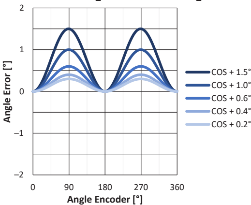
Figure 13: Angle Error from Cosine Phase Error
