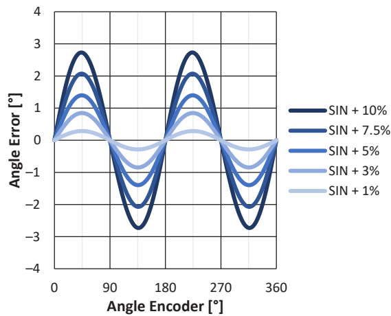
Figure 10: Angle Error from Sine Amplitude Mismatch
