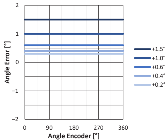
Figure 14: Angle Error from Equal Phase Error
