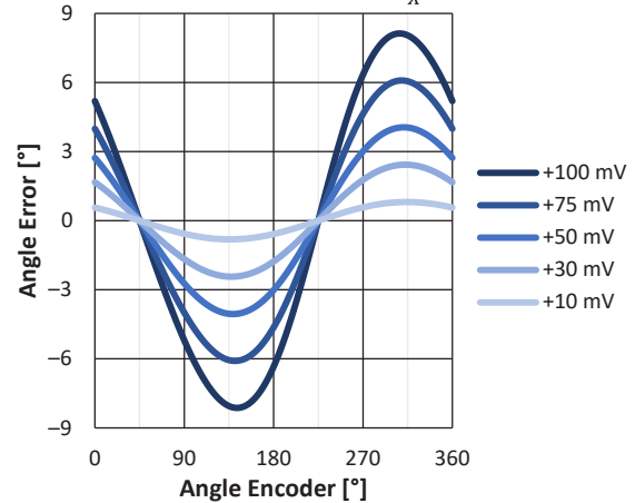
Figure 9: Angle Error from Equal Sine and Cosine Offset Error
