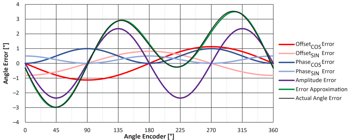
Figure 15: Approximation of Angle Error versus Actual Angle Error
