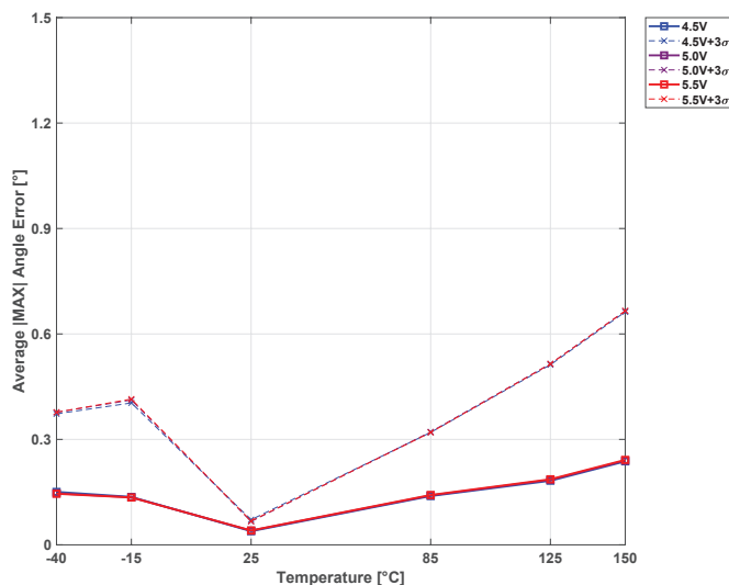
Figure 21: A33230 Average |Max| Dynamic Correction Angle Error +3σ over Temperature and Vcc
