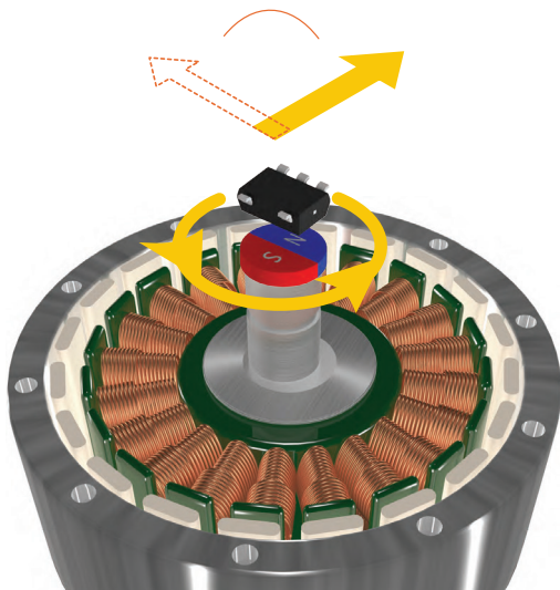
Figure 1: End-of-Shaft Rotary Position Application
