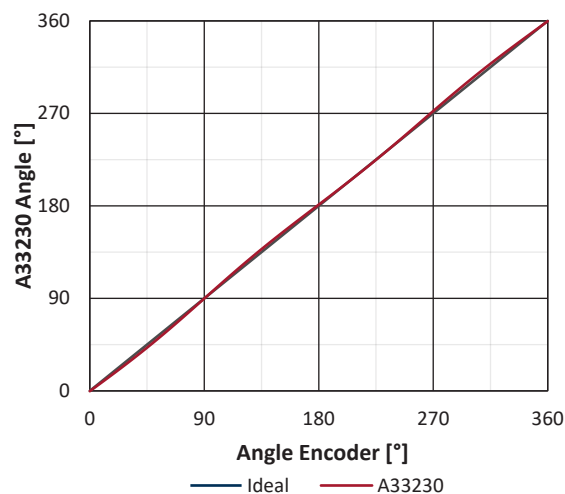
Figure 4: Normalized Device Angle versus Reference Angle
