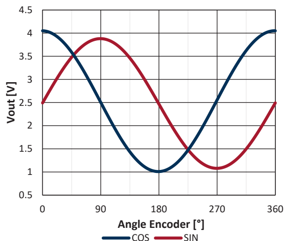
Figure 2: Native Sine/Cosine Outputs
