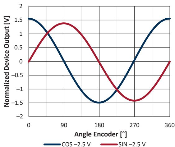
Figure 3: Output with Ideal Offset Removed
