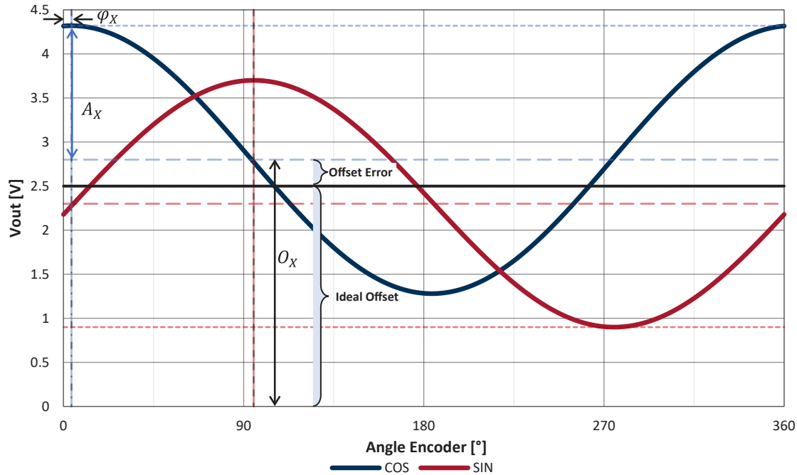
Figure 6: Understanding Offset ( O ), Amplitude ( A ), and Phase ( \varphi )
