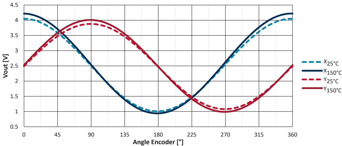
Figure 16: Example OutputA (X), OutputB (Y) Signals at 25^\circ\text{C} and 150^\circ\text{C}
