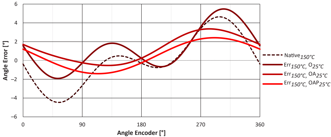
Figure 19: Native Error versus Error at 150°C after Application of 25°C Offset, Amplitude, and Phase Correction
