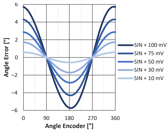
Figure 7: Angle Error from Sine Offset Error
