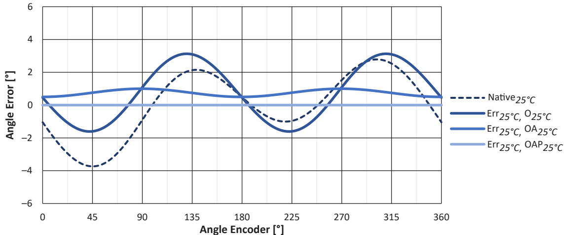
Figure 18: Native Error versus Error at 25°C after 25°C Offset, Amplitude, and Phase Correction
