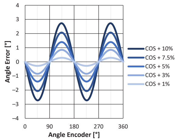
Figure 11: Angle Error from Cosine Amplitude Mismatch
