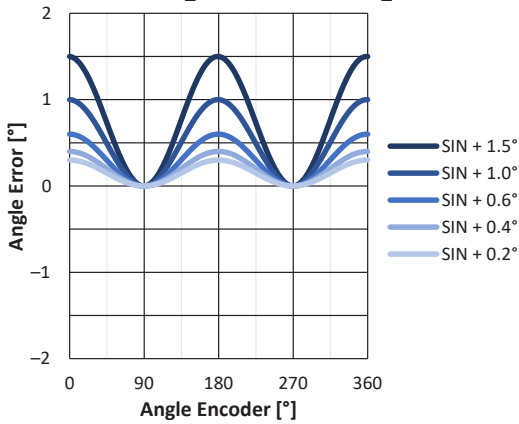
Figure 12: Angle Error from Sine Phase Error
