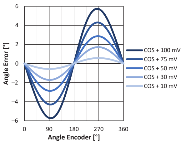
Figure 8: Angle Error from Cosine Offset Error
