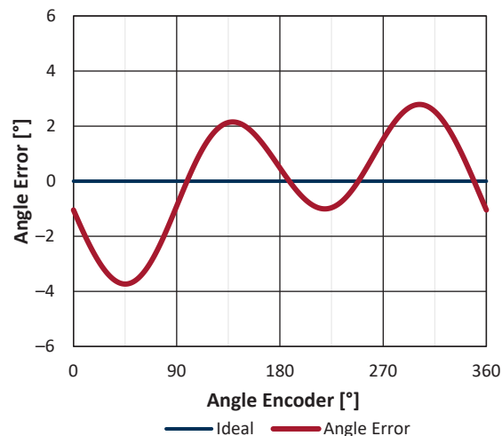
Figure 5: Normalized Native Angle Error
