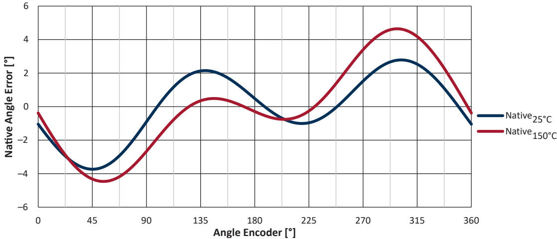
Figure 17: Angle Error After 2.5 V Offset Correction (Native Angle Error)
