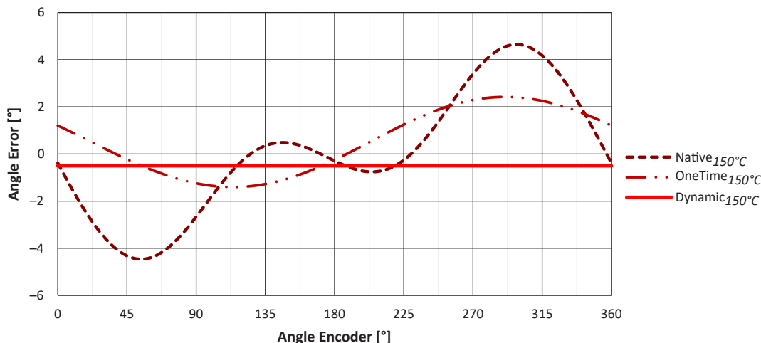
Figure 20: Comparison of Native Error, One-Time 25°C Correction Error, and Dynamic Error at 150°C
